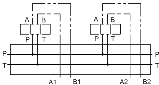
Hydraulic Circuit
